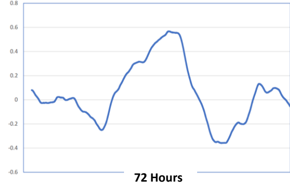
Smoothed raw data, all GCP events
