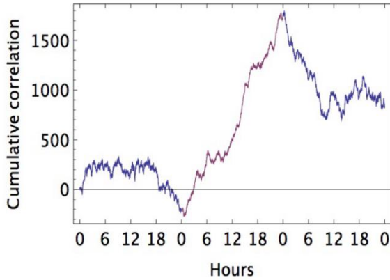
Cumulative deviation, all GCP events
