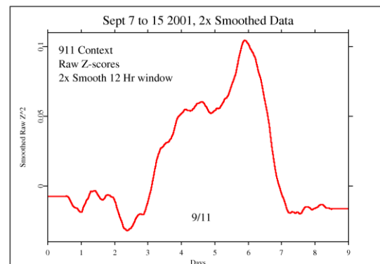
Smoothed raw data for 9 days around 9/11
