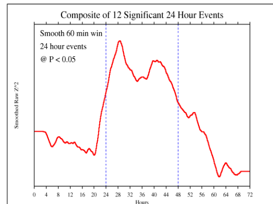
Signal Averaged GCP Event Response
