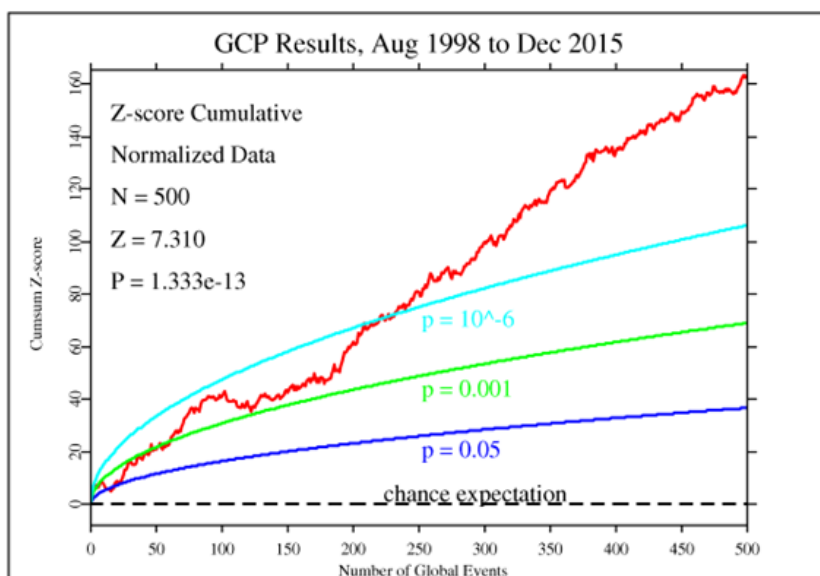
Figure 1. Graphical summary of the experimental results accumulated by the Global Consciousness Project with its worldwide network of RNGs over the course of 500 event database from August 1998 to December 2015.
