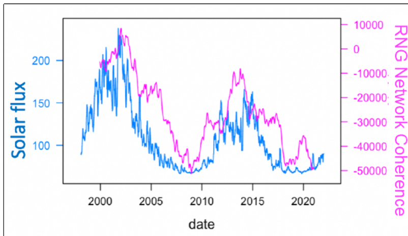
Figure 3. Time series data of the intensity of F10.7 solar radio flux compared to the long-term trend data from GCP 1.
